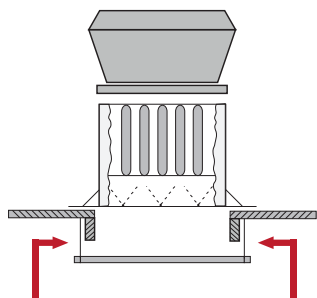
MDV with sound absorbing plate
